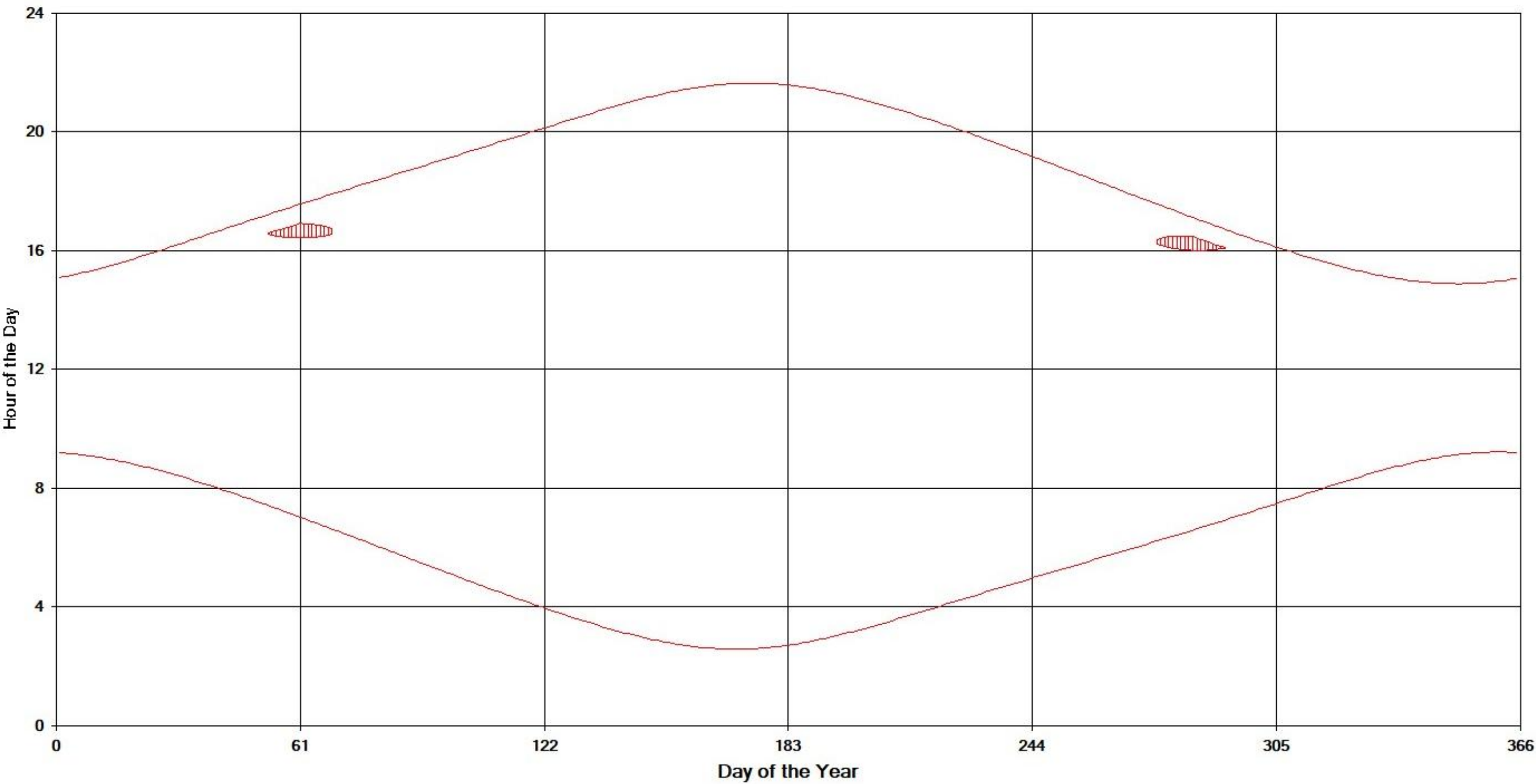
Graph 1: Potential shadow flicker times on House 1, all windows from all turbines
