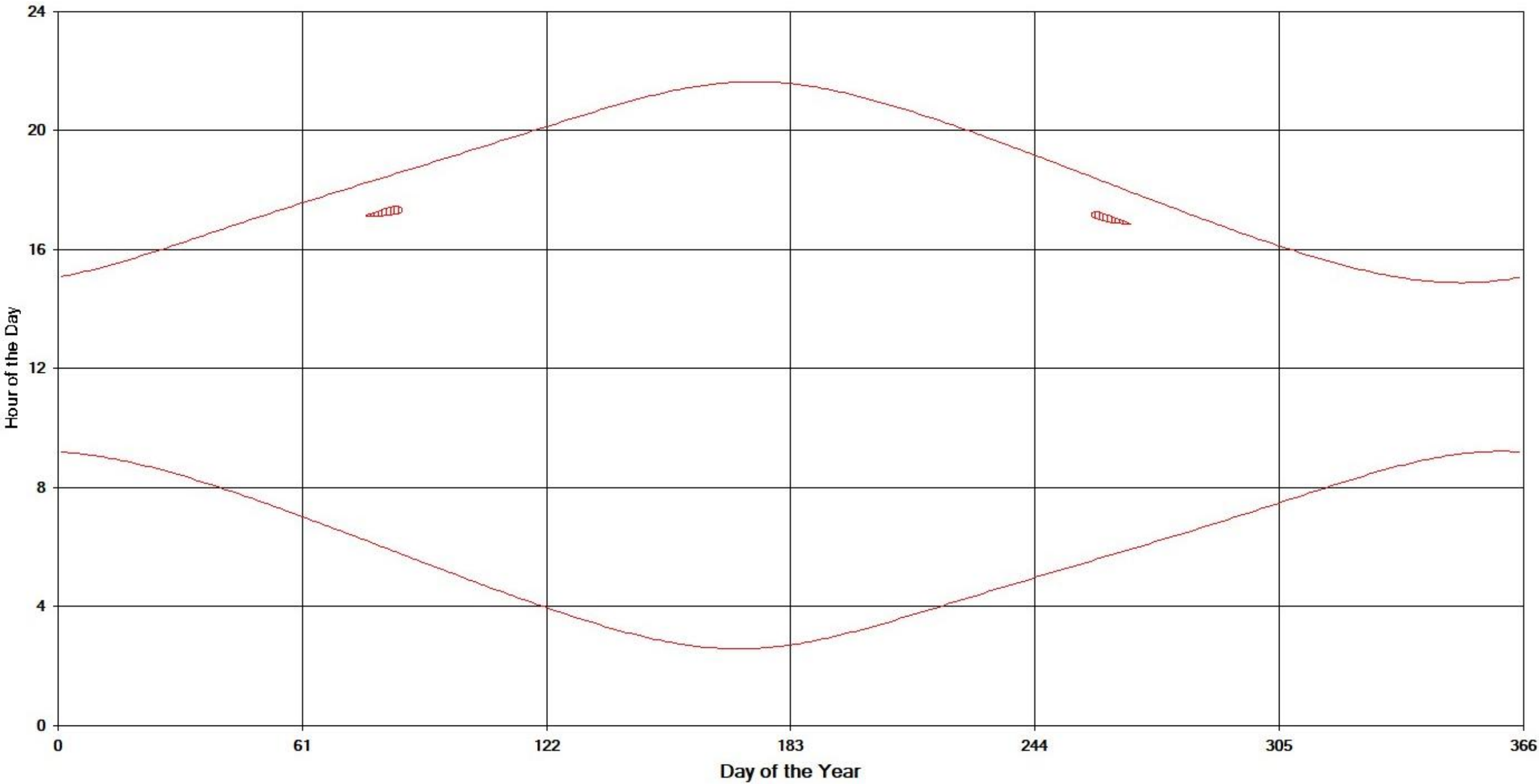
Graph 4: Potential shadow flicker times on House 4, all windows from all turbines
