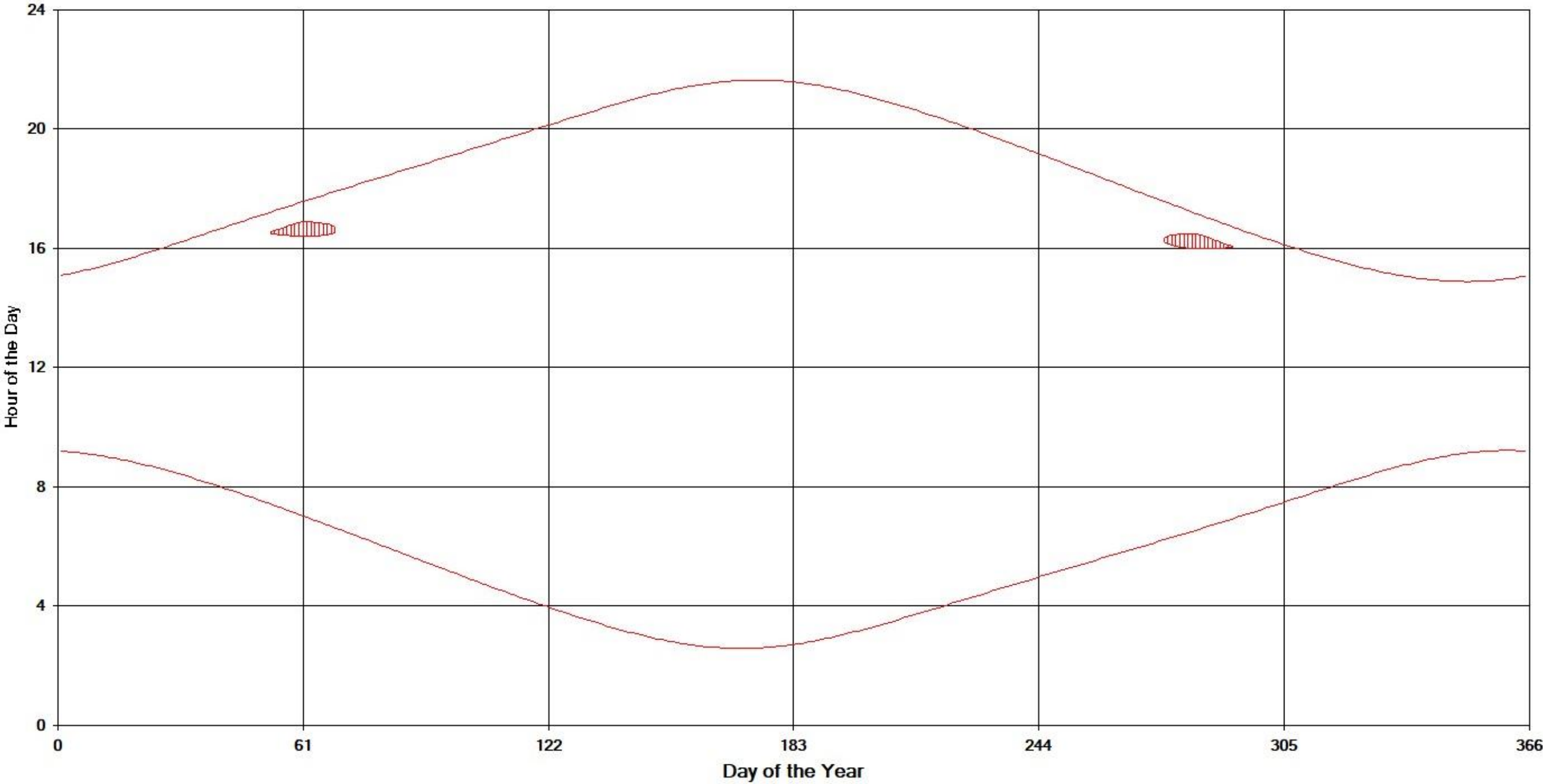
Graph 2: Potential shadow flicker times on House 2, all windows from all turbines
