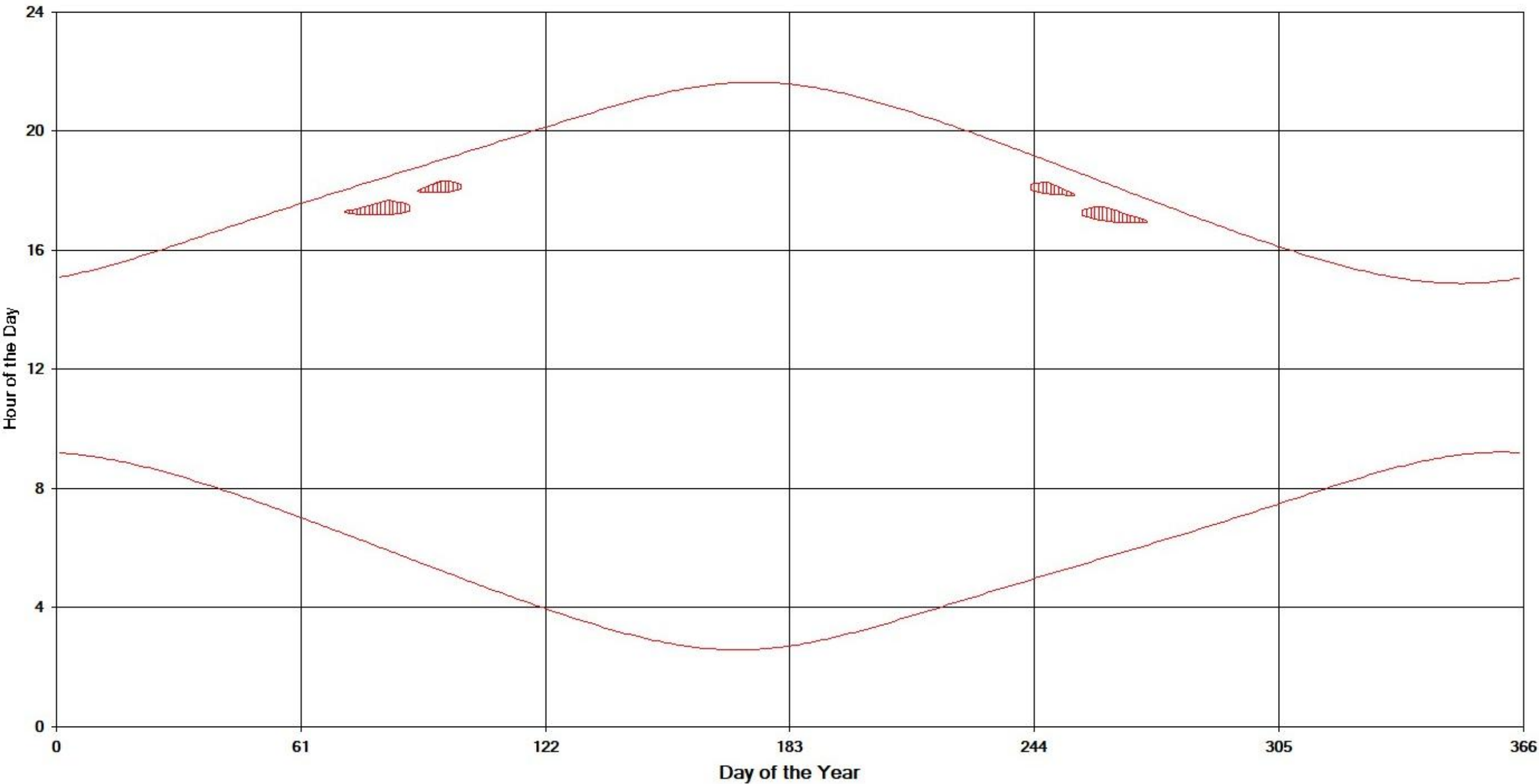
Graph 5: Potential shadow flicker times on House 5, all windows from all turbines
