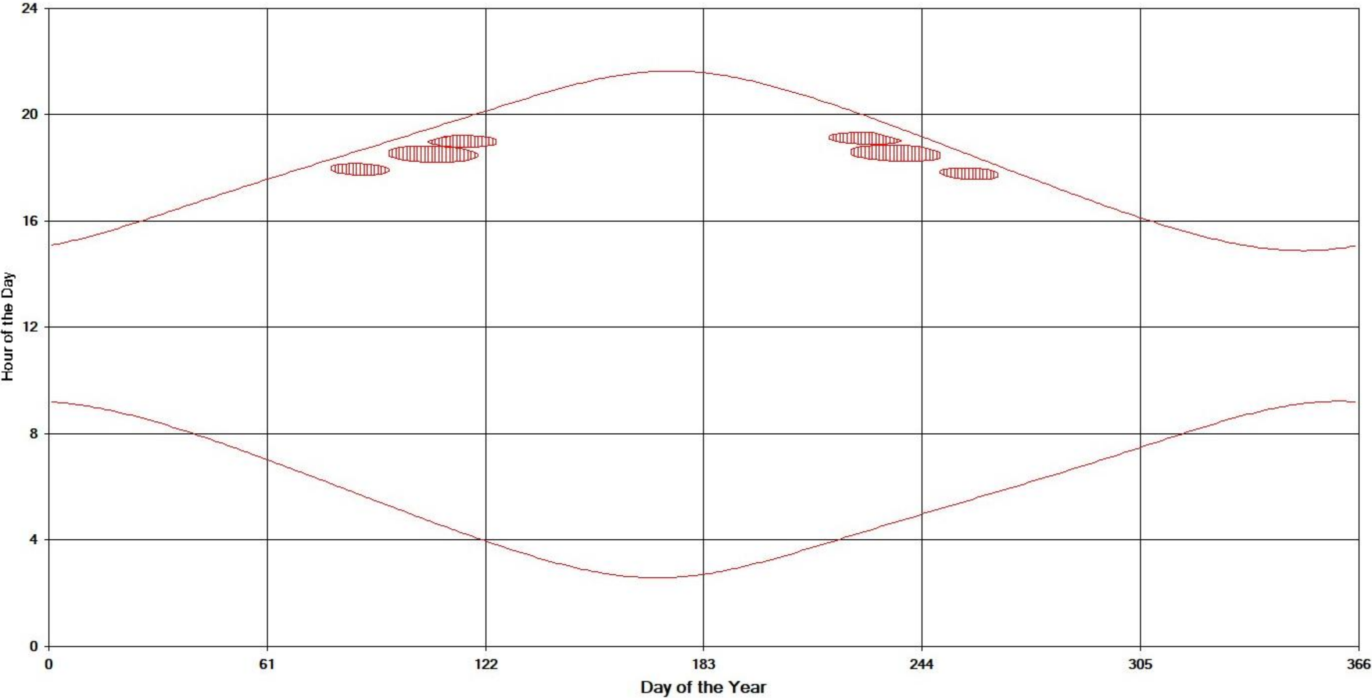
Graph 8: Potential shadow flicker times on House 8, all windows from all turbines
