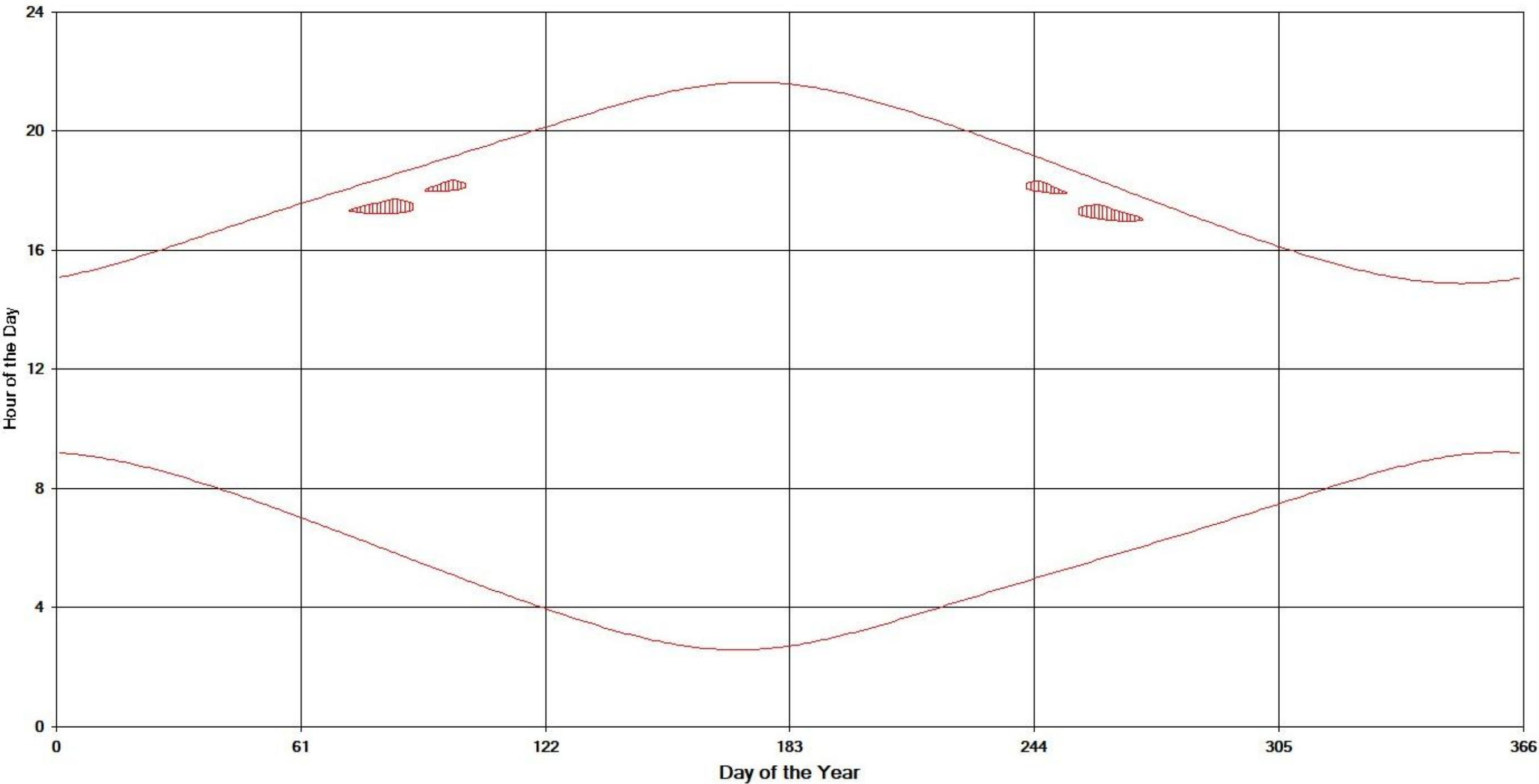
Graph 6: Potential shadow flicker times on House 6, all windows from all turbines
